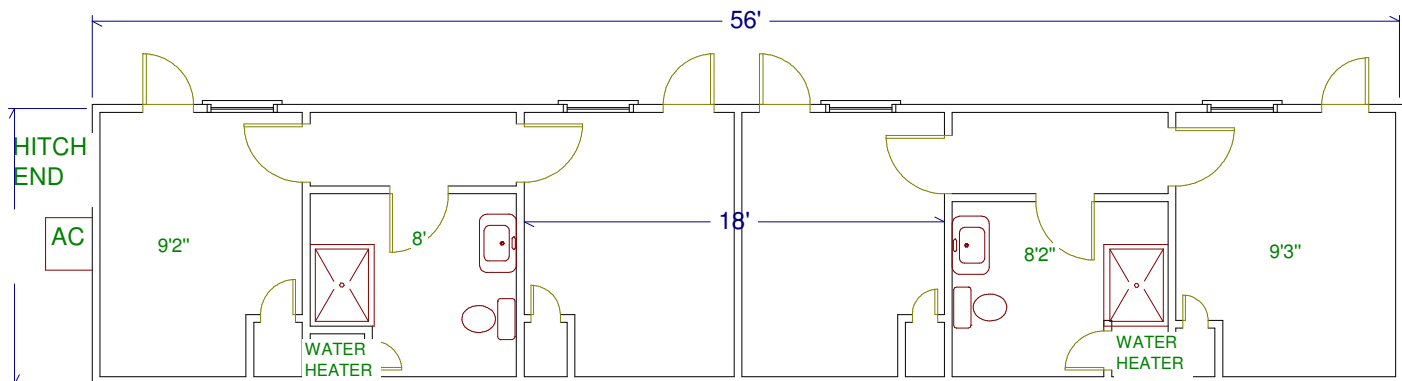
12 X 56 BUNKHOUSE
